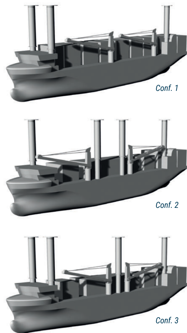
Figure 1: 3D Geometry of three configurations for the Flettner rotor installation on a MPV Vessel
