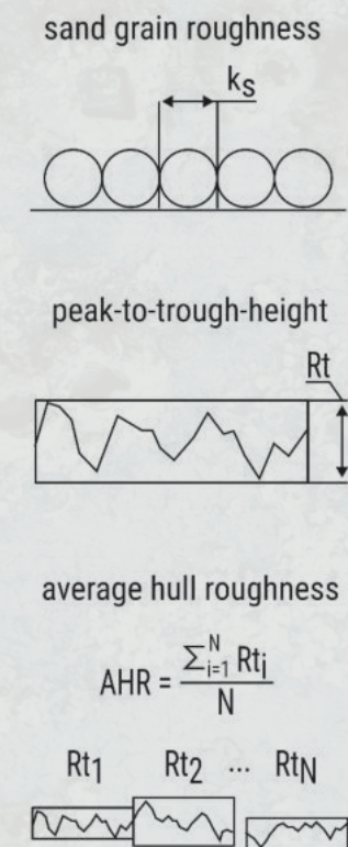
Figure 1: Different roughness definitions
